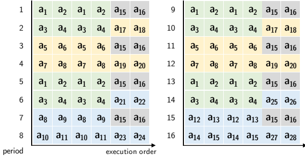
Fig. 19: A frequency-based pattern. Example of a frequency-based pattern with \mathcal{T} = 6 , pattern length 96, and 16 periods. Aggressors are colored based on their frequency f : \frac{1}{2} (blue), \frac{1}{4} (green), \frac{1}{8} (yellow), \frac{1}{16} (orange).
