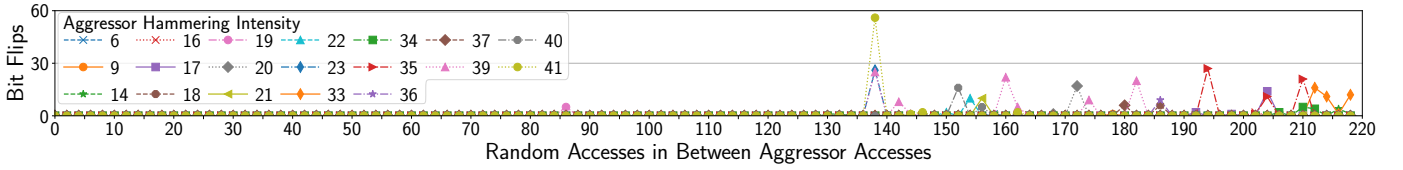
Fig. 8: Hammering duration. Observed bit flips on B_2 for patterns up to three REFRESH intervals, a varying number of random accesses and aggressor hammering intensities. Choosing an offset of 138 with intensity of 41 triggers the most (56) bit flips. We omit intensities without any bit flips.
