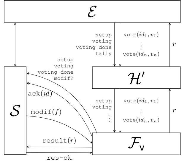
Figure 4. The ideal execution with id_1, \dots, id_n \in H
