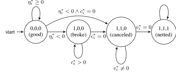
Fig. 4: Inventory flags state transition diagram
