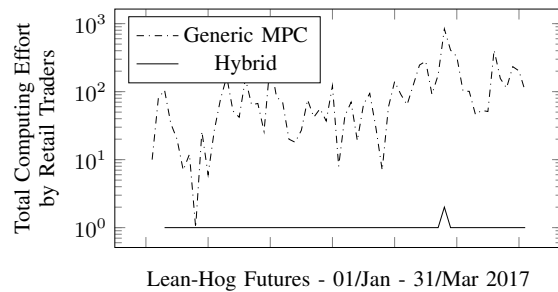
With MPC retail traders have to always participate whether they make an order or not (and they overwhelmingly don't [41]). They would be supplying to algorithmic traders some orders of magnitude of costly computing resources. With our approach the burden on retail traders is significantly smaller.
