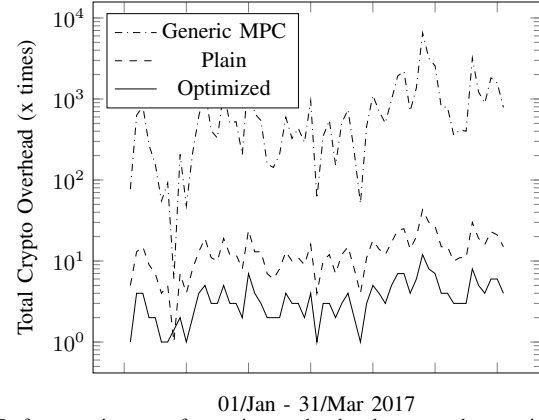
Performance in terms of execution overhead to the expected processing time (1 day). For the optimized version, only one day of trading exhibits overheads greater than 10x and only ten days greater than 5x. These overheads could be already offset by parallelizing the traders ZK-proofs (each trader has to do several of them) which would yield an improvement factor of 6x.
