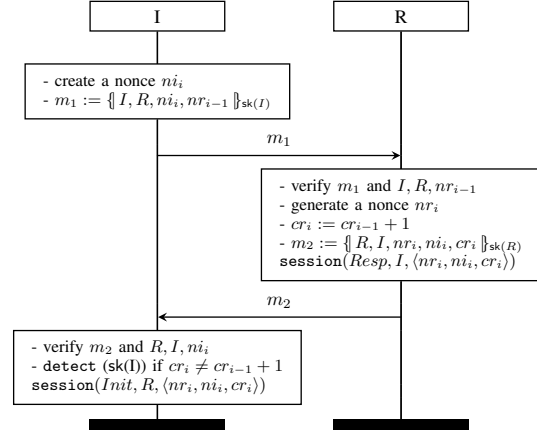
Fig. 2. The counter protocol. The inclusion of nr_{i-1} in m_1 could instead be provided as a nonce in an additional message m_0 = \{R, I, nr_i\}_{sk(R)} , as in the Keyless SSL example in Figure 3
