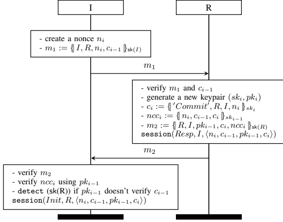
Fig. 4. A commitment protocol.
