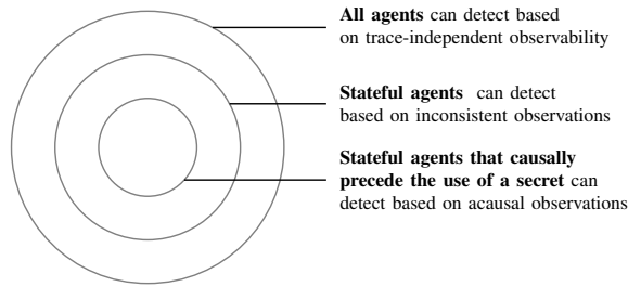
Fig. 1. Venn Diagram of the type of agents and the detection mechanisms that they might be able to use. Only stateful agents that causally precede the use of a secret can use all three types.
