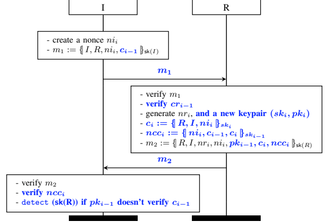
Fig. 5. The i -th session of the modified ISO-IEC 9798-3-3 standard protocol. Modifications are highlighted in bold blue.
