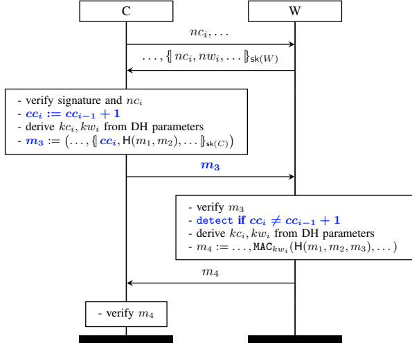
Fig. 3. An example of the additions to the i -th session of the TLS mutually-authenticated key exchange in Keyless SSL. For clarity, we omit terms in the messages that are not relevant. Our modifications are highlighted in bold blue.
