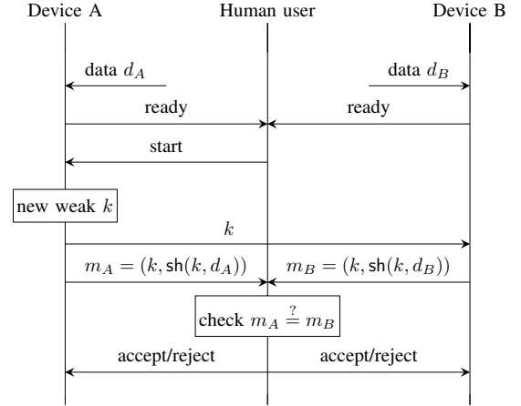
Fig. 6. Manual authentication mechanism 2 from [23]
