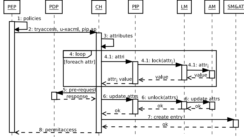
Fig. 3. Sequence Diagram for Pre-Authorization
