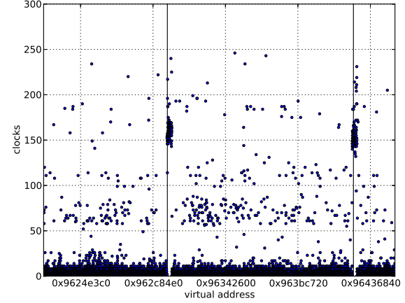
Figure 7. Extract of cache preloading measurements
