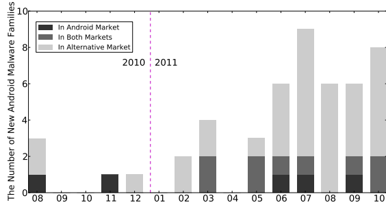
(a) The Monthly Breakdown of New Android Malware Families
