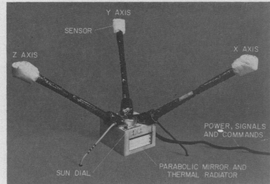
Fig. 1. Lunar surface magnetometer as deployed on the moon. The sensors are at the top end of the booms and approximately 70 cm above the lunar surface. The electronics and motor drive assembly are located in the box, encased in a thermal blanket. Heat rejection during lunar day and retention during lunar night are controlled by a parabolic reflector array on two sides of the electronics box. The astronaut bubble level and azimuthal shadow-graph are shown on top of the box. Power, digital signals, and commands are provided through the ribbon cable which connects to the ALSEP central-station telemetry receiver and transmitter.
