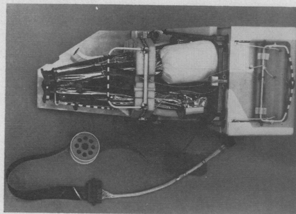
Fig. 11. The lunar surface magnetometer in stowed configuration.
