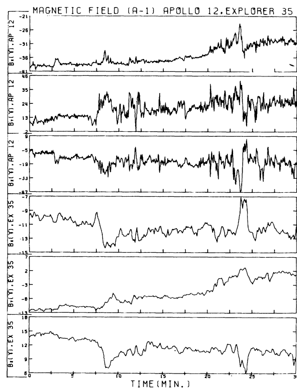
Fig. 18. Simultaneous time-series magnetic-field data from the Apollo 12 magnetometer and the lunar-orbiting Explorer 35 satellite while the moon is located inside the earth's magnetosheath. Data are plotted in a lunar surface coordinate system which is oriented with x toward the zenith, y east, and z north.
