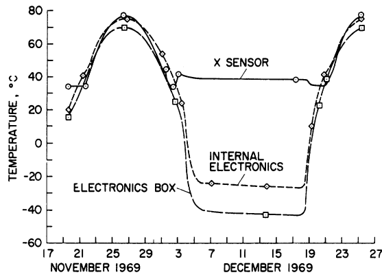
Fig. 12. Temperatures inside the magnetometer during the first postdeployment lunation. The sun was directly overhead at the magnetometer site on November 26; sunset occurred on December 4, and sunrise on December 18.
