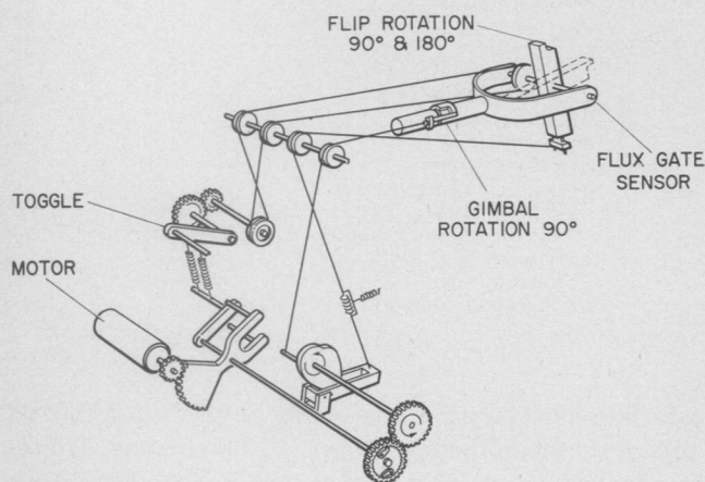
Fig. 10. Mechanical gimbal and sensor-flip unit.
