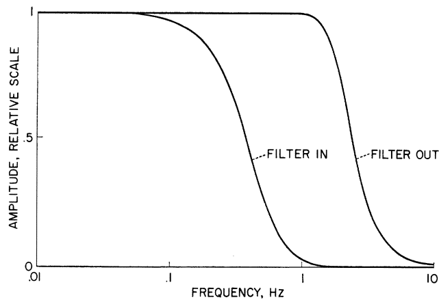
Fig. 5. Frequency response of the lunar surface magnetometer electronics, as measured through the telemetry link, with the digital filter in the circuit and with the digital filter bypassed.
