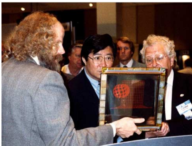
Fig. 21. Energy recovery sustain circuit developed at the University of Illinois in 1986 was used in this prototype [34]. This circuit is used in all of today's TV products to reduce the set power by more than 100 W.
