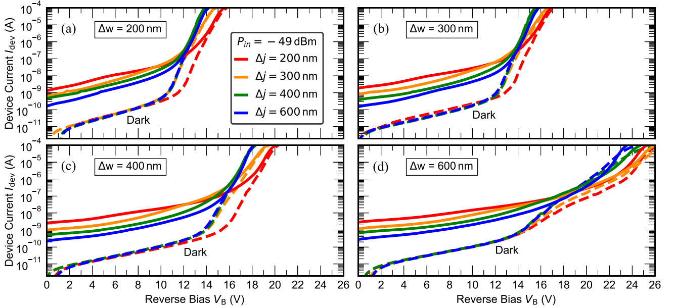
Fig. 3. Current-voltage (I-V) characteristics of all device variants. Each subfigure shows devices with the same intrinsic region width \Delta w , but different intrinsic region displacement \Delta j . Solid lines show measurements with input optical power P_{in} = -49 dBm (after accounting for insertion losses); dashed lines show dark current I_{dark} . All subfigures share the same legend.
