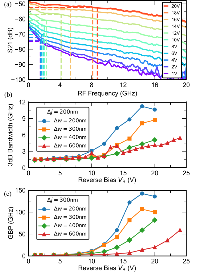
Fig. 6. RF performance of the PIN devices. (a) RF response at different reverse bias V_B for a device with \{\Delta w, \Delta j\} = \{200, 300\} nm. Dashed lines indicate the 3 dB rolloff point with respect to the reference frequency of 1 GHz. (b) 3 dB bandwidth for devices with \Delta j = 200 nm. (c) Gain-bandwidth product (GBP) for devices with \Delta j = 300 nm. The input power is P_{\text{in}} = -7.4 dBm for all plots in this figure.
