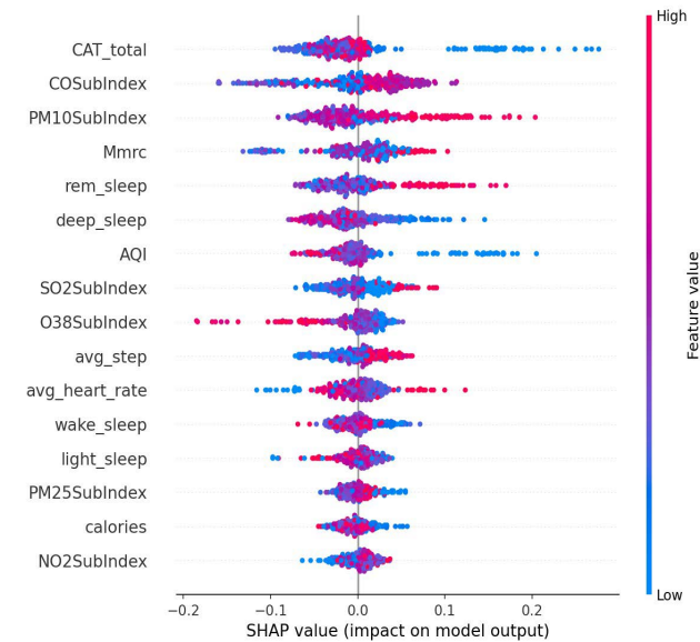
FIGURE 14. Summary plot of AECOPD model.
