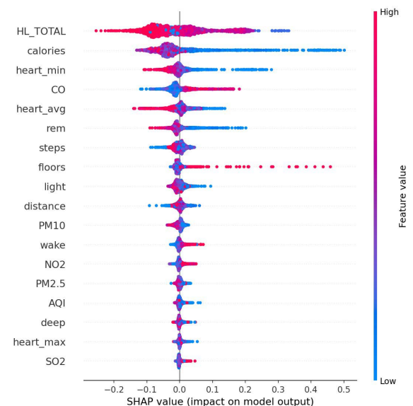
FIGURE 20. Summary plot of obesity model.
