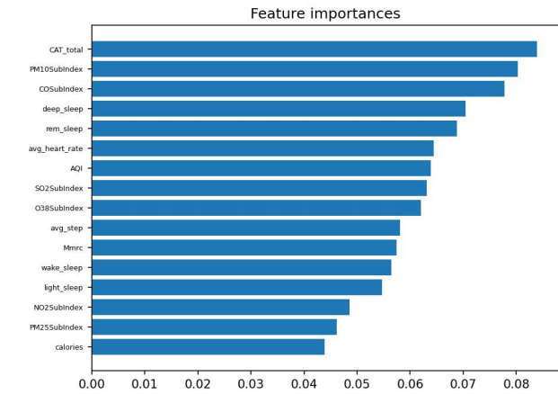
FIGURE 13. Feature importance scores of AECOPD model.
