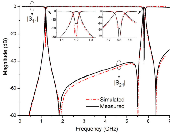
FIGURE 11. Simulated and measured results of Filter I.
