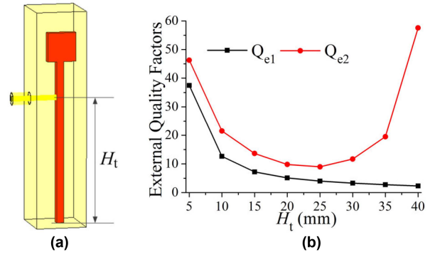
FIGURE 15. (a) Feeding structure. (b) The external quality factors of the first two resonant modes against H_t .
