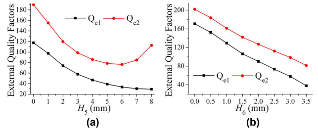
FIGURE 6. (a) The external quality factors of the first two resonant modes against H_5 with fixed H_6 = 3 mm. (b) The external quality factors of the first two resonant modes against H_6 with fixed H_5 = 4 mm.
