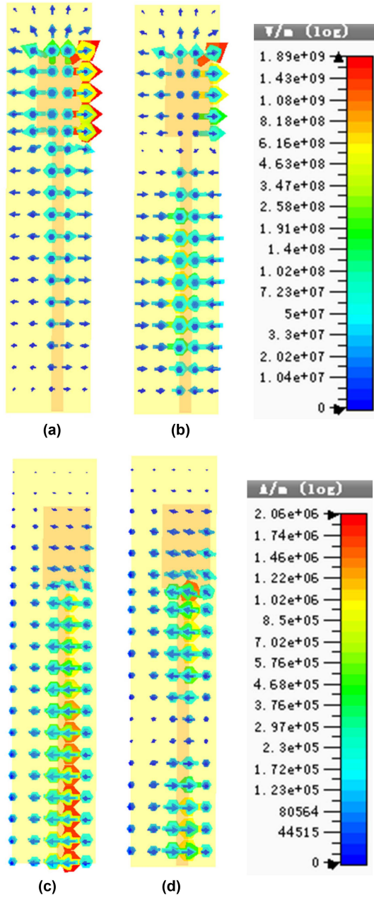
FIGURE 13. (a) E-field of the fundamental mode. (b) E-field of the second mode. (c) B-field of the fundamental mode. (d) B-field of the second mode.
