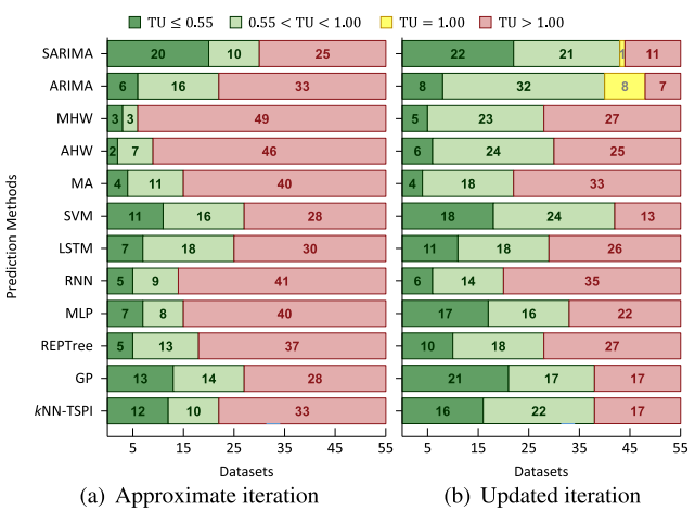
FIGURE 19. Performance, in terms of TU, of the state-of-the-art methods across the 55 datasets.
