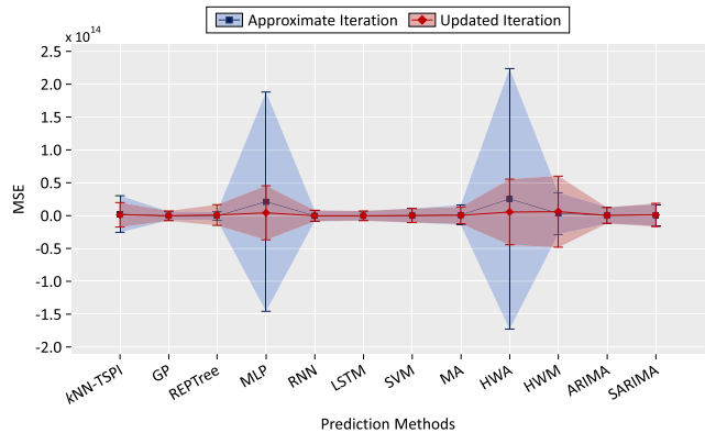
FIGURE 18. Averages and SD of MSE obtained by the state-of-the-art methods.
