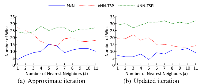
FIGURE 17. Number of wins achieved by each similarity-based predictor given 55 datasets and the variation of parameter k from 1 to 11.
