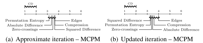
FIGURE 27. MPCM derived from k NN-TSPI configured with various complexity measures.
