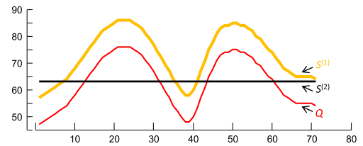
FIGURE 7. Example of variance to amplitude and offset. Popular distances measures such as Euclidean and DTW indicate that Q is more similar to S^{(2)} than S^{(1)} .
