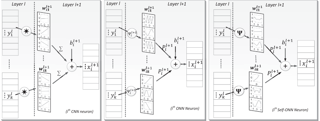
Fig. 1. An illustration of the 1D nodal operations with the 1D kernels of the k^h CNN (left), ONN (middle), and Self ONN (right) neurons at layer l/[54] .
