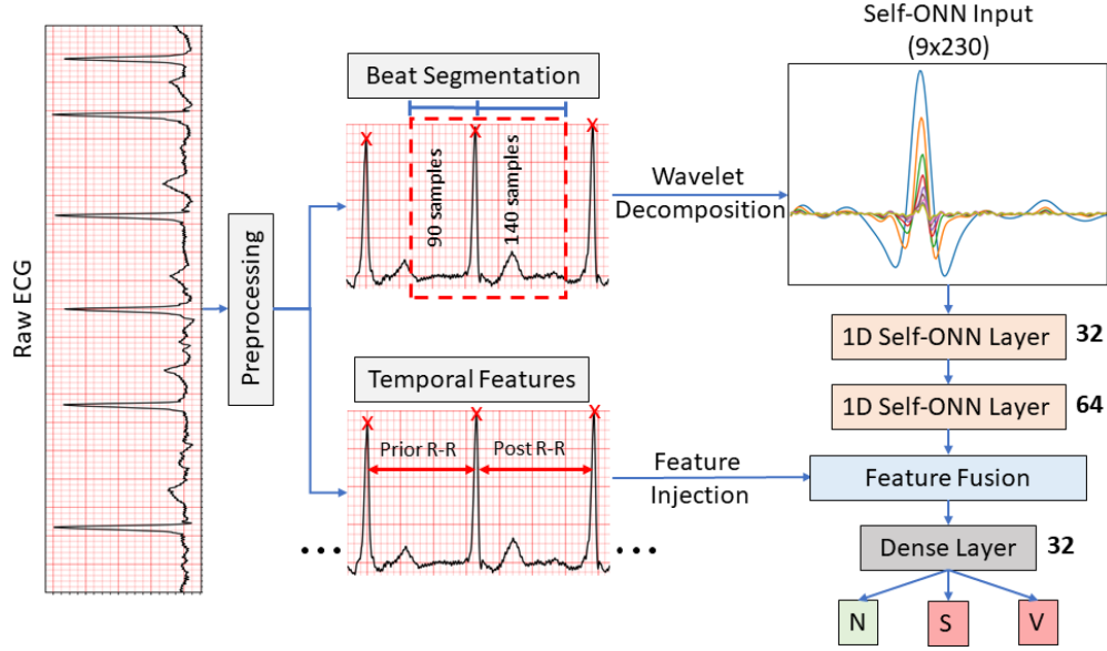
Fig. 2. Block diagram of the proposed approach and model architecture for classification of ECG signals.
