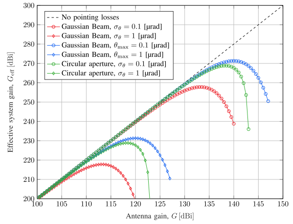
Fig. 2. Effective system gain (23) versus the antenna gain G = G_t = G_r . Deterministic ( \theta_{\text{max}} -based) and probabilistic ( \sigma_{\theta} -based) approaches; P_{\text{out}} = 5\% when probabilistic approach is employed; different values of the pointing accuracy parameters; Gaussian beam and circular aperture models.
