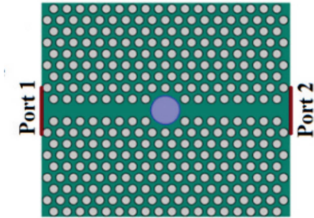
FIGURE 6. Illustrates a cross-section of the 2D PhC biosensor with the central microcavity filled with glucose solution [74].
