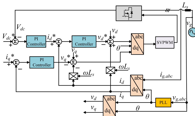
FIGURE 11. Control method of a three-phase boost rectifier based on d-q axis transformation.
