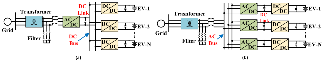
FIGURE 3. Architecture of an EV off-board charging station: (a) DC connected system. (b) AC connected system.
