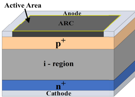
Fig. 2. Cross section of the studied Si p-i-n photodiodes (photodetectors).
