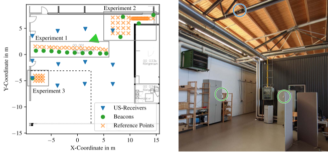
Fig. 5. Left: Experiments Overview. The first experiment is concerned with estimating the performance of linear constrained localization with BLE, whereas the second demonstrates the efficacy of using BLE data to directly enhance the TDOA solution. The point of view of the right figure is marked with the green triangle. Right: View of the second experiment. The US-receiver (blue) is mounted at a height of 4.8 m. The two foremost Bluetooth beacons (green) are visible, which are installed at a height of 1.6 m. The left figure shows the corresponding point of view.
