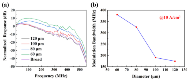
Fig. 5. (a) Frequency responses and (b) bandwidth of the 120, 100, 80, and 60 \mu\text{m} micro-LED arrays.
