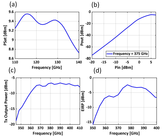
Fig. 15. Transmitting chain simulated performance. (a) Frequency doubler saturated power versus frequency. (b) Frequency tripler output power versus input power at output frequency of 375 GHz. (c) Transmitter chain output power versus frequency. (d) EIRP versus frequency of the Tx Chain.
