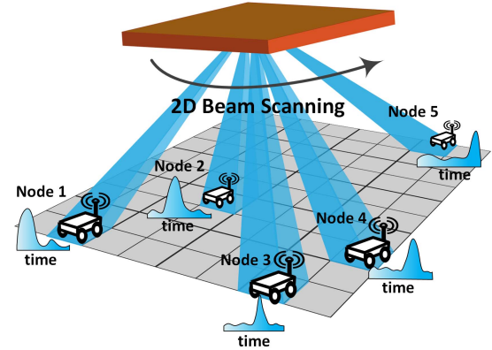
Fig. 1. Conventional node localization approach with directive beams at mmWave/THz showing beam-optimization across multiple links established through iterative scanning in 2-D space.
