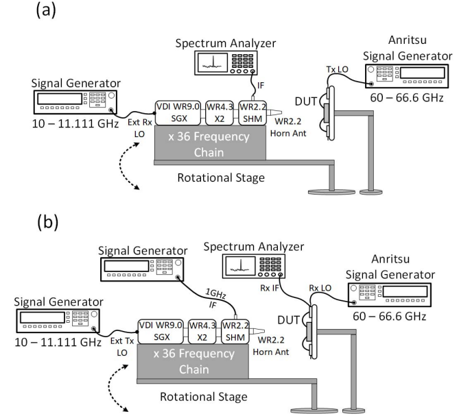
Fig. 21. THz transceiver characterization. (a) Far-field measurement setup of the on-chip transmitter. (b) Far-field measurement setup of the on-chip receiver.
