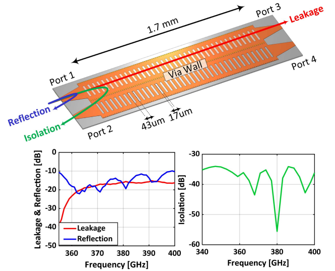
Fig. 12. Simulated scattering parameters of the two dual-port LWA across the frequency.
