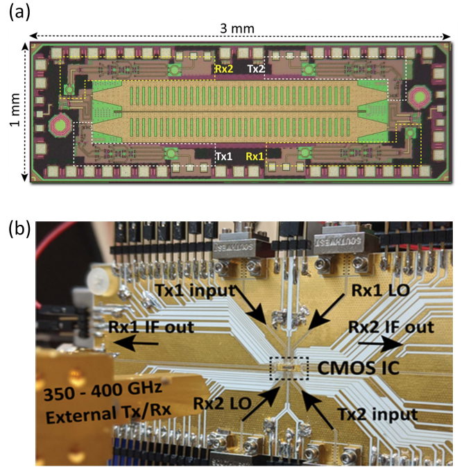
Fig. 20. THz Prism chip and packaged photograph. (a) Chip micrograph of the THz Prism occupying 3 mm². (b) Chip packaging and external connectors.
