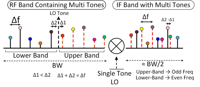
Fig. 19. Setting the LO frequency at the center of the received tones with a slight offset, the lower and the upper band tones can be uniquely decoded by the receiver.
