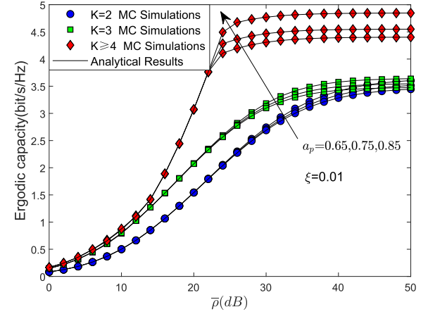
FIGURE 7. EC of the system versus different K and different a_p : FHS.
