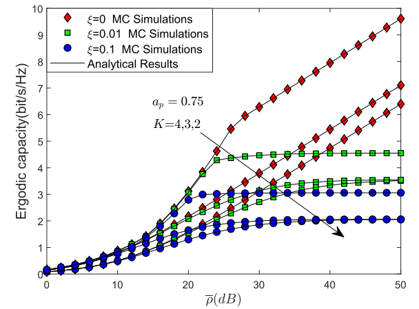
FIGURE 8. EC of the system versus different K and different \xi : FHS.
