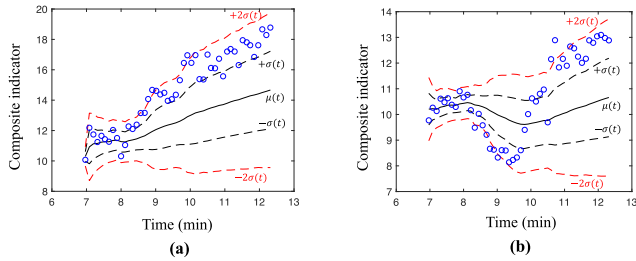
Fig. 8. Composite early warning index comprising all three indicators extracted from velocity measurements (left) and density measurements (right) in the empirical US-101 highway case study.
