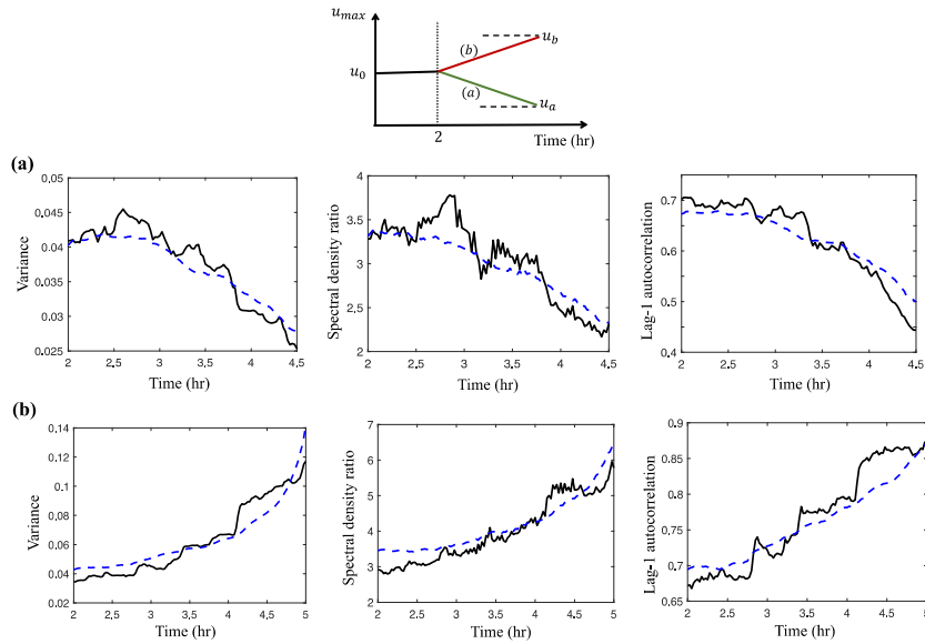
Fig. 5. Measurable changes in the trend of the early warning signals at a fixed mean density and a progressive (a) decrease and (b) increase in the maximum allowed driving speeds. The solid black lines represent the EWSs obtained from a single 500m segment of the road, and the dashed blue lines show the average of the EWSs obtained from all road segments.
