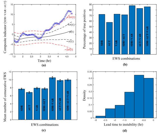
Fig. 4. (a) Example of the constructed composite signal combining standardized variance ( Var ), lag-1 autocorrelation ( AUT ) and spectral density ratio ( SDR ) plotted against time. The blue circles show the composite signal, and the running average ( \mu ) and standard deviation boundaries ( \sigma and 2\sigma ) are also marked in the figure. A passage of the 2\sigma threshold by the composite index represents a slowing down in the dynamics. (b) Percentage of the true positives, i.e. the composite index passes the 2\sigma threshold for five consecutive time steps, for each combination of the EWSs obtained from 400 independent simulations of the traffic flow dynamics exhibiting instability. (c) Mean number of maximum consecutive passages of the 2\sigma threshold for each combination of EWSs. (d) Distribution of the remaining time to a traffic jam when the composite indicator W = Var + AUT + SDR predicts an imminent instability based on the 2\sigma criteria.
