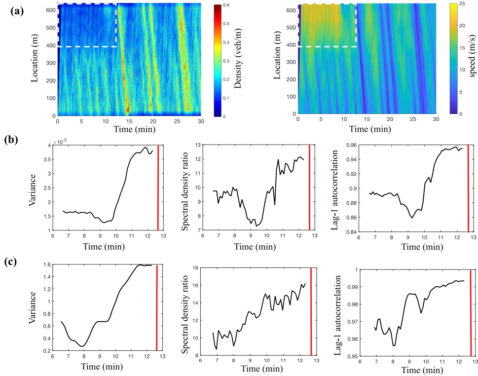
Fig. 7. Early warning signals of traffic congestions for US-101 highway. (a) Spatio-temporal evolution of density and velocity of vehicles on the road for the first 30 minutes of the recordings. The measurements used to extract early warning signals is depicted by a dashed box in the plots. (b) Early warning signals obtained from density measurements. (c) Early warning signals obtained from velocity measurements. Vertical red line shows the time at which the traffic instability is observed. (d) Composite early warning index comprising all three indicators extracted from velocity measurements (left) and density measurements (right) in the empirical US-101 highway case study.
