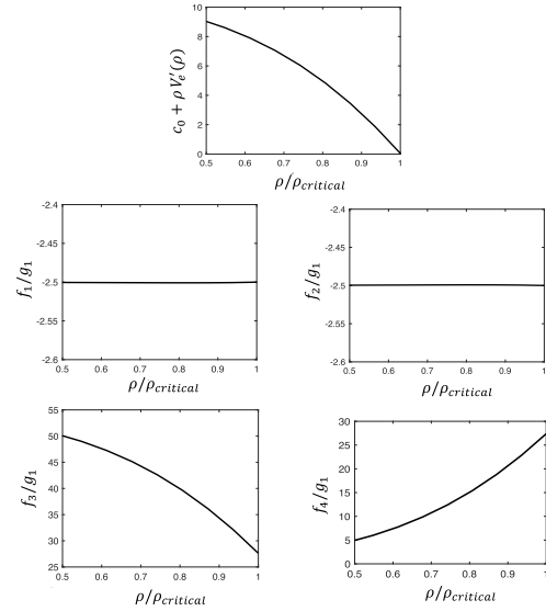
Fig. 10. Trends of the functions appeared in Eq. (12) computed for the model parameters described in Methods and varying \rho as the control parameter.
