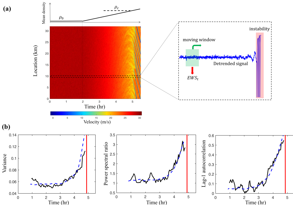
Fig. 2. Early warning signals of traffic instability in a highway with periodic boundary conditions. (a) Spatiotemporal pattern of the traffic flow velocity under a change in the mean density. The mean car density on the road is stationary for the first simulated two hours and increases linearly afterward to reach to its critical value. Patterns of upstream stop and go traffic jam are observed when the dynamics passes its stability threshold. (b) Early warning signals of loss of the traffic stability and resilience obtained from stochastic fluctuations in the measured mean velocity of cars at selected road segments. In each graph, the solid black line is the EWS obtained from a single 500m segment of the road, the dashed blue line is the average of the EWSs obtained from all road segments, and the vertical red line shows the time at which the traffic instability is observed.
