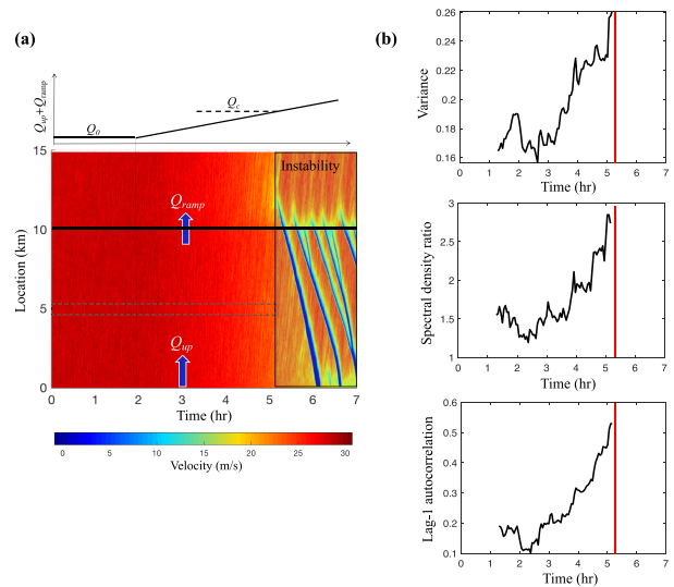
Fig. 6. Early warning signals of traffic instability in a highway with an on-ramp. (a) Spatiotemporal pattern of the traffic flow velocity under the change of the inflow to the road. The traffic inflow is stationary for the first simulated two hours and increases linearly afterward to reach its critical value. (b) Early warning signals of loss of the traffic stability and resilience obtained from stochastic fluctuations in the measured mean velocity of cars at selected road segments (schematically shown with a horizontal box in the figure). The vertical red line shows the time at which the traffic instability is observed.
