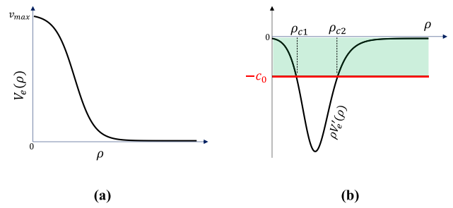
Fig. 9. Schematic of (a) the fundamental velocity function ( V_e ) and (b) the resulting stability boundaries obtained in Eq. (5). The stable region is marked with green color.
