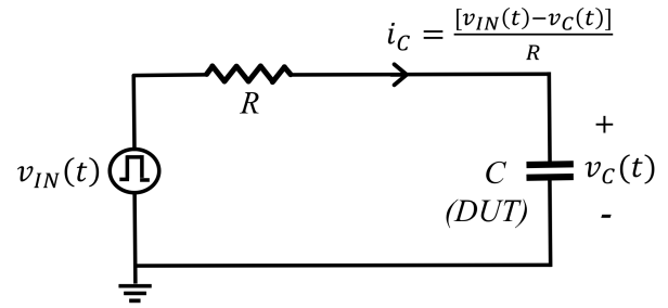
FIGURE 1. Measurement circuit with the MOS capacitor (C) as the device under test (DUT) and an external series resistor R .
