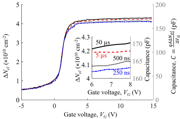
FIGURE 5. Electron-density change ( \Delta N_{el} ) and capacitance corresponding to gate-voltage steps \Delta V_G = 100 mV. In the inset, the solid, the dashed, the dotted, and the dash-dot lines correspond to the electrons responding the gate-voltage steps within time intervals of 50 \mu s, 5 \mu s, 500 ns, and 250 ns, respectively.
