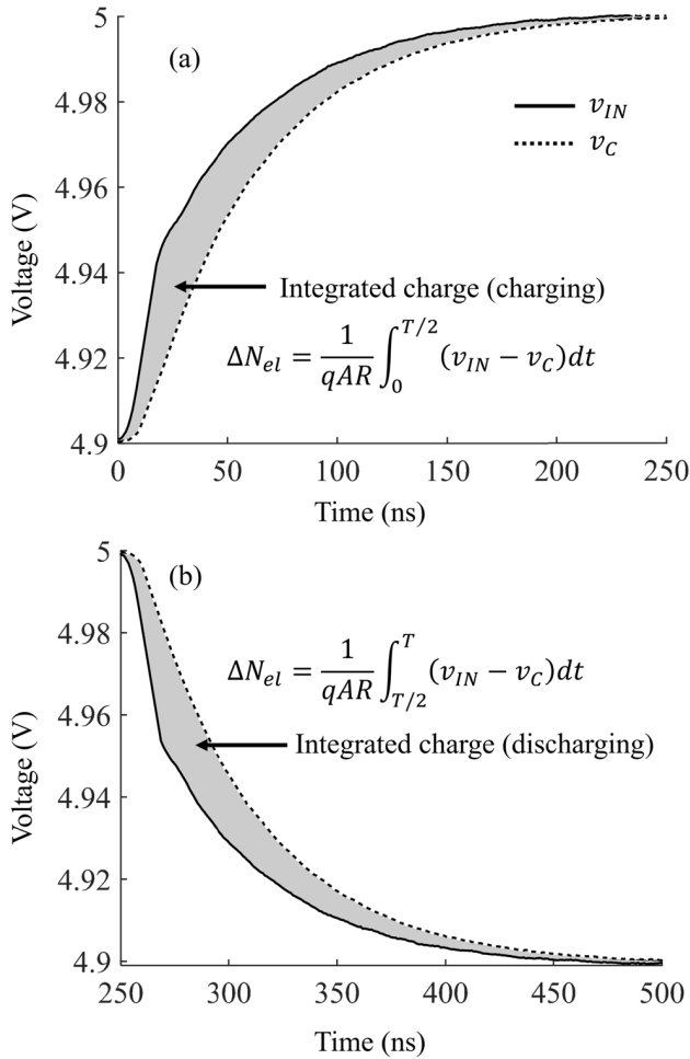
FIGURE 2. Illustrative voltage transients: (a) rising edge for charging, (b) falling edge for discharging. The voltage transients consist of real data measured at V_G = 4.95\text{ V} with 2 MHz rectangular waveform (the digital storage oscilloscope automatically averages thousands of periods to deliver these traces over a single period).
