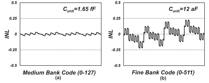
Fig. 11. Simulated INL of (a) medium bank and (b) fine bank.
