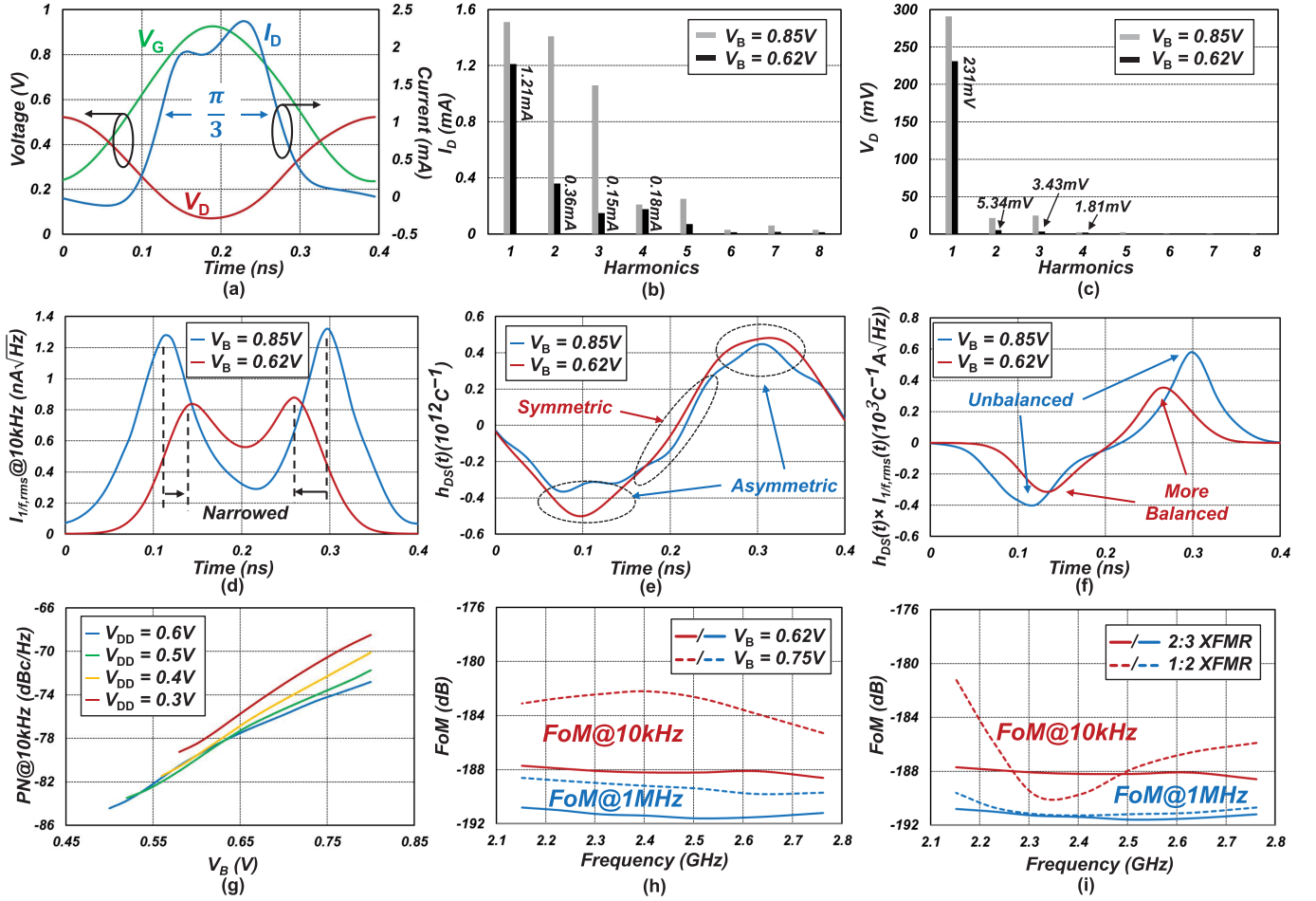
Fig. 6. (a) Simulated waveforms of V_G , V_D , and I_D when V_B = 0.62 V. Spectral harmonics of (b) I_D and (c) V_D at different V_B . Time evolution plots of: (d) 1/f noise current intensity ( i_{1/f,rms} @ 10 kHz), (e) ISF transfer function h_{DS} , and (f) effective ISF ( h_{DS} \times i_{1/f,rms} @ 10 kHz) at different V_B at 0.3 V supply. (g) Simulated PN plots at 10 kHz versus V_B at different supply levels. (h) FoM@10 kHz and FoM@1 MHz versus carrier frequency when V_B = 0.62 V and V_B = 0.75 V and (i) comparison of FoM of 2:3 and 1:2 transformers versus carrier frequency, when V_B of 1:2 transformer is 0.62 V and V_B of 2:3 transformer is 0.65 V.
