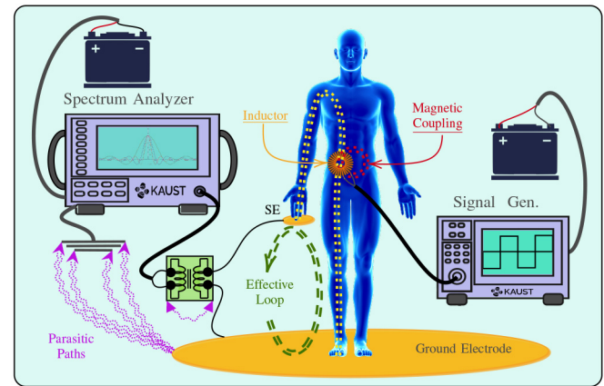
Fig. 8. Illustration of MC-based HBC.
