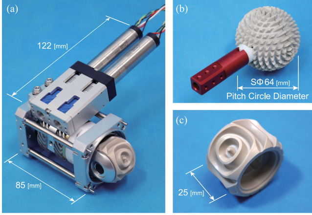
Fig. 13. Main components of the manufactured prototype. (a) Driving gear. (b) CS-gear and output link. (c) MP-gear.
