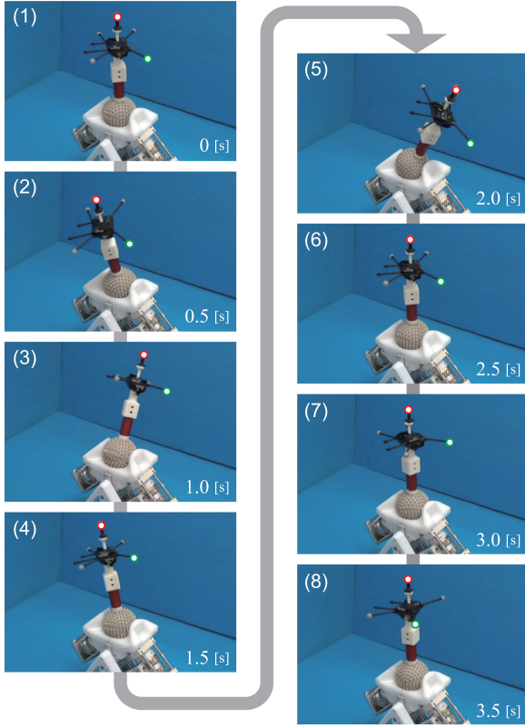
Fig. 19. Movement of the prototype of the new ABENICS in the tracking experiment. To clarify the movement, two infrared reflection markers were characterized with simple red and green circles in these pictures.
