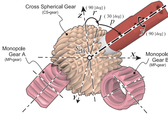
Fig. 21. Schematic diagram of the CS-gear and MP-gears of the perpendicular type prototype at the CS-gear orientation r = 90 [deg] p = 30 [deg], and y = 90 [deg]. Note that the coordinate axes in this figure are in the right-hand coordinate system, i.e., this view is from the minus side of the Z-coordinate. In this case, the roll rotation r of the CS-gear is performed by the gearing motion of both the MP-gears.
