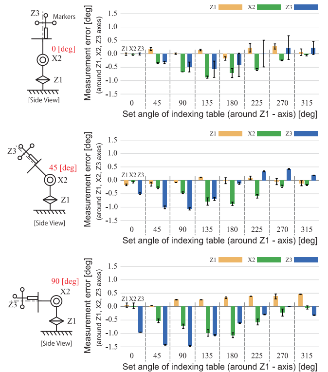
Fig. 25. Accuracy of 3D measuring equipment. Z1 was set at 0–360 in 45 [deg] increments, and X2 was set at 0, 45, and 90 [deg]. The graph is the average of the two measurements and the error bars indicate the difference. In each measurement, the values were taken after standing still for 20 s.
