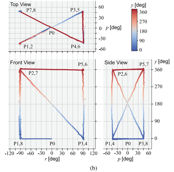
Fig. 20. Scatterplot of the tracking experiment results. XYZ-Euler angles (roll r , pitch p , and yaw y [deg]) are plotted in the Cartesian coordinate system. The color of the plotted points illustrates the angle of y [deg] and the linearity of the plotted points indicates the transient response of this mechanism. (a) Perspective view. (b) Three-view.
