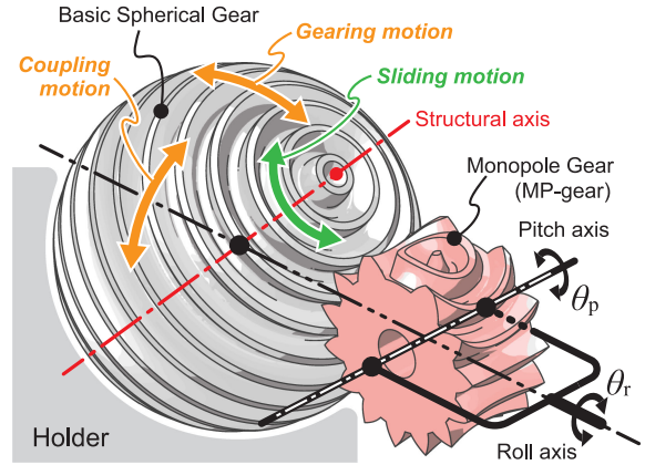
Fig. 8. Three motions are invoked by the interaction between the MP-gear and the CS-gear.
