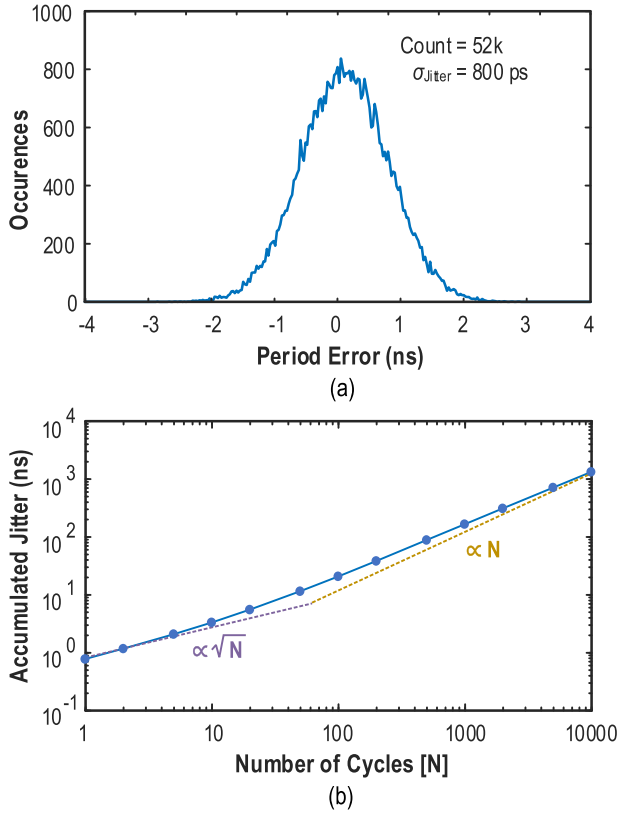
Fig. 10. (a) Measured period jitter of the RxO (52 000 hits on the oscilloscope). (b) Accumulated jitter of the RxO.
