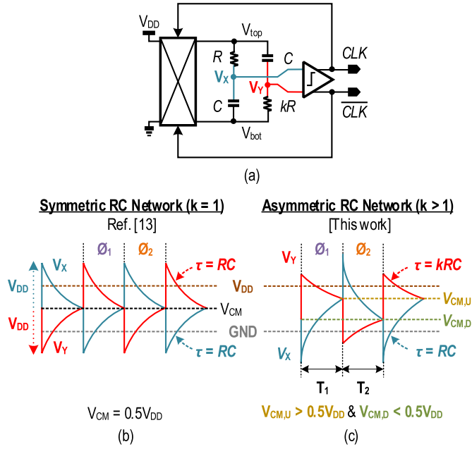
Fig. 1. (a) Simplified schematic of the swing-booster differential RxO. (b) Timing diagram of the output of the RC network with k=1 , where V_{CM} is fixed at 0.5V_{DD} . (c) Timing diagram of the output of the RC network with k>1 , such that V_{CM,U} and V_{CM,D} suit the design of the subsequent ULV comparator (this work).
