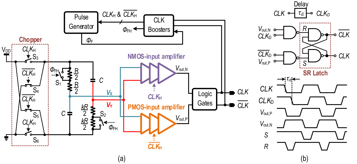
Fig. 3. (a) Proposed ULV swing-boostered RxO featuring an asymmetric RC network and a dual-path comparator. The delays of the amplifiers are tracked to tackle the frequency fluctuation against temperature and voltage variations. (b) Schematic of the logic gates. The SR latch, together with the delay unit, guarantees that the RxO only generates desired oscillating signal without glitch.
