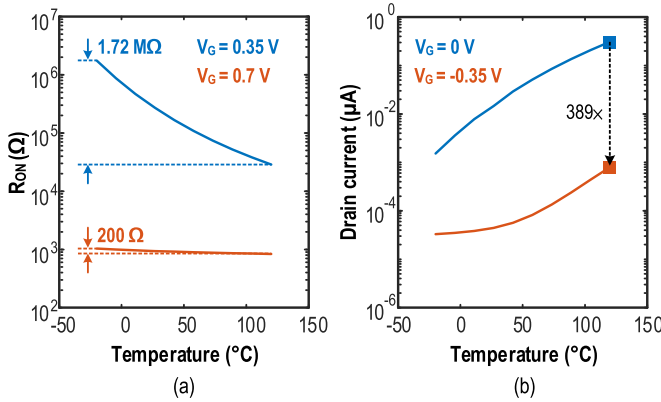
Fig. 7. (a) R_{ON} of an NMOS from -20 to 120 °C with different V_G . For both cases, V_D = V_S = 0.175 V. The increased swing on V_G reduces the variations of R_{ON} by 8600×. (b) I_{Leak} of the same NMOS in the OFF-state. With a negative V_G , the I_{Leak} is reduced by 389× at 120 °C. For both cases, V_D = 0.35 V and V_S = 0 V.
