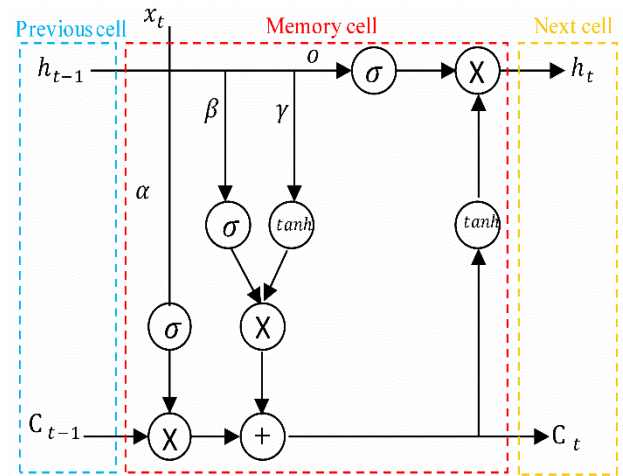
FIGURE 5. LSTM-Memory cell.
