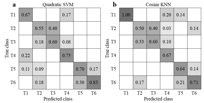
FIGURE 10. The confusion matrix of six touch behaviors using quadratic SVM (a) and cosine KNN (b), respectively.
