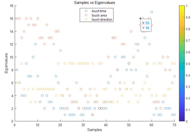
FIGURE 9. Visualization of partial touch samples containing three touch characteristics (time, area and direction), showing that the features are not linearly separable.
