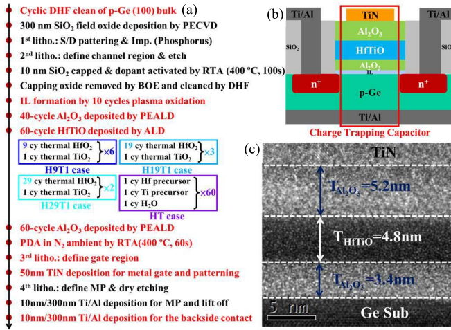
FIGURE 1. (a) Process flow of CTCs and CTMTs. The process steps of CTC are colored in red. (b) Illustration of the structure of CTC and CTMT. The structure of CTC is framed by red line. (c) TEM image of the gate stack.
