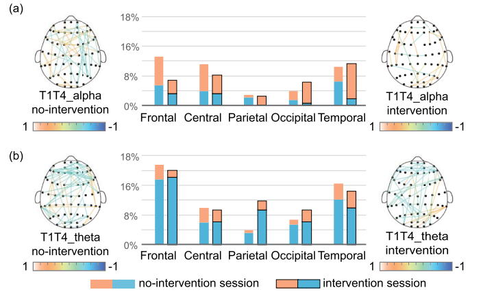
Fig. 4. The selected discriminative features in the general effect classification (i.e., T1 vs. T4). (a) The percentage of increased and decreased FC in the alpha band. The color bars indicate the different weights of FC. The negative values indicate the decreased FC and the positive values indicate the increased FC. (b) The percentage of increased and decreased FC in the theta band. The yellow boxes represent the increased connectivity, and blue boxes represent the decreased connectivity.
