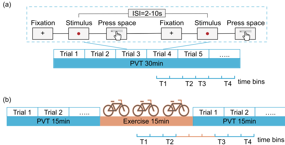
Fig. 1. The experimental paradigm. (a) Participants performed a 30-min PVT in the no-intervention session . Each participant was asked to press the space bar as soon as possible when the red stimulus appeared. The inter-stimulus interval (ISI) is a random value in the range of 2 - 10s. The 30-min PVT was divided into six 5-min time bins, T1 and T4 correspond to the first and last time bins, respectively. T2 and T3 correspond to the two time bins in the middle. (b) In the intervention session , participants were required to perform a 15-min cycling in the middle of the PVT execution. The PVT before and after the exercise intervention was divided into 5-min time bins, T2 and T3 correspond to the pre- and post-intervention time bins, respectively.
