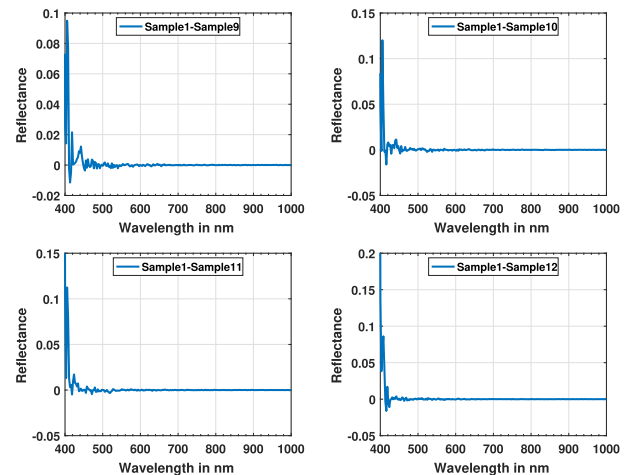
FIGURE 8. Mean spectra of PCA (a) Sample 1 - 9 (b) Sample 1 - 10 (c) Sample 1 - 11 (d) Sample 1 - 12.
