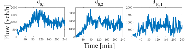
Fig. 4. Traffic demand used in the simulation experiments.
