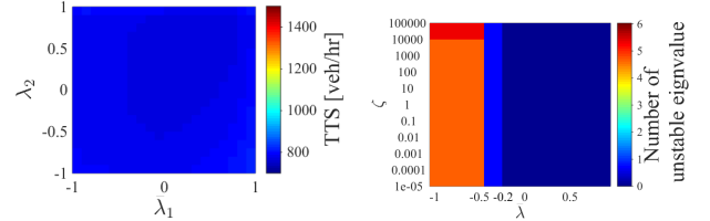
Fig. 8. TTS for a domain of \lambda_1 and \lambda_2 (left) and number of negative eigenvalues in \Theta (right), while w_Q = 1 , w_{R_1} = 1 , and w_{R_2} = 0.001 .
