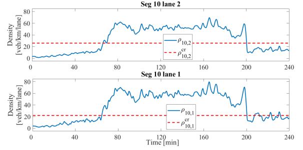
Fig. 6. Density at bottleneck cells in the no-control case.
