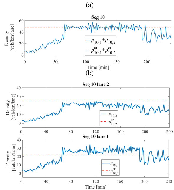
Fig. 14. Density at bottleneck cells in the ALINEA controlled case. (a) Summation of densities at bottlenecks, (b) Separated value of density at bottleneck cells.
