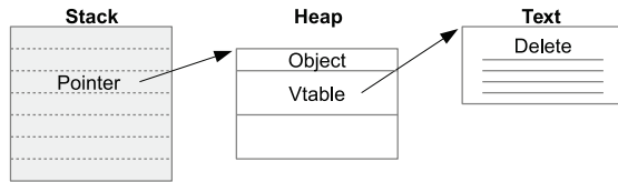
(a) In an object's first deletion, the call to delete is correctly looked up in the vtable of the object.
