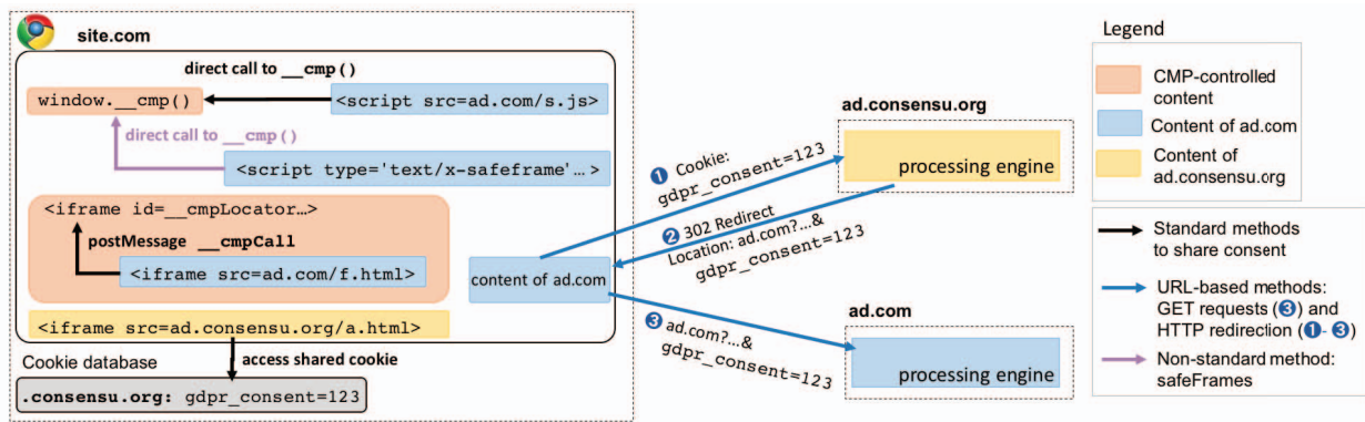
Fig. 3: The methods to share consent in IAB Europe’s TCF.
