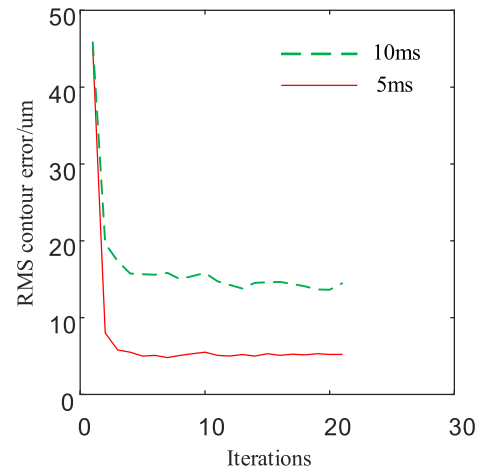
FIGURE 16. Comparison of time-varying RMS errors with control periods of 10ms and 5ms (experiment).
