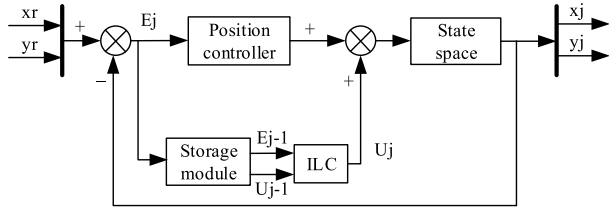
FIGURE 2. Iterative learning control block diagram.
