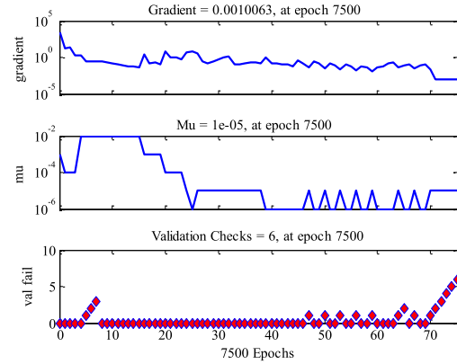
FIGURE 9. Performance evolution of deep learning neural network.
