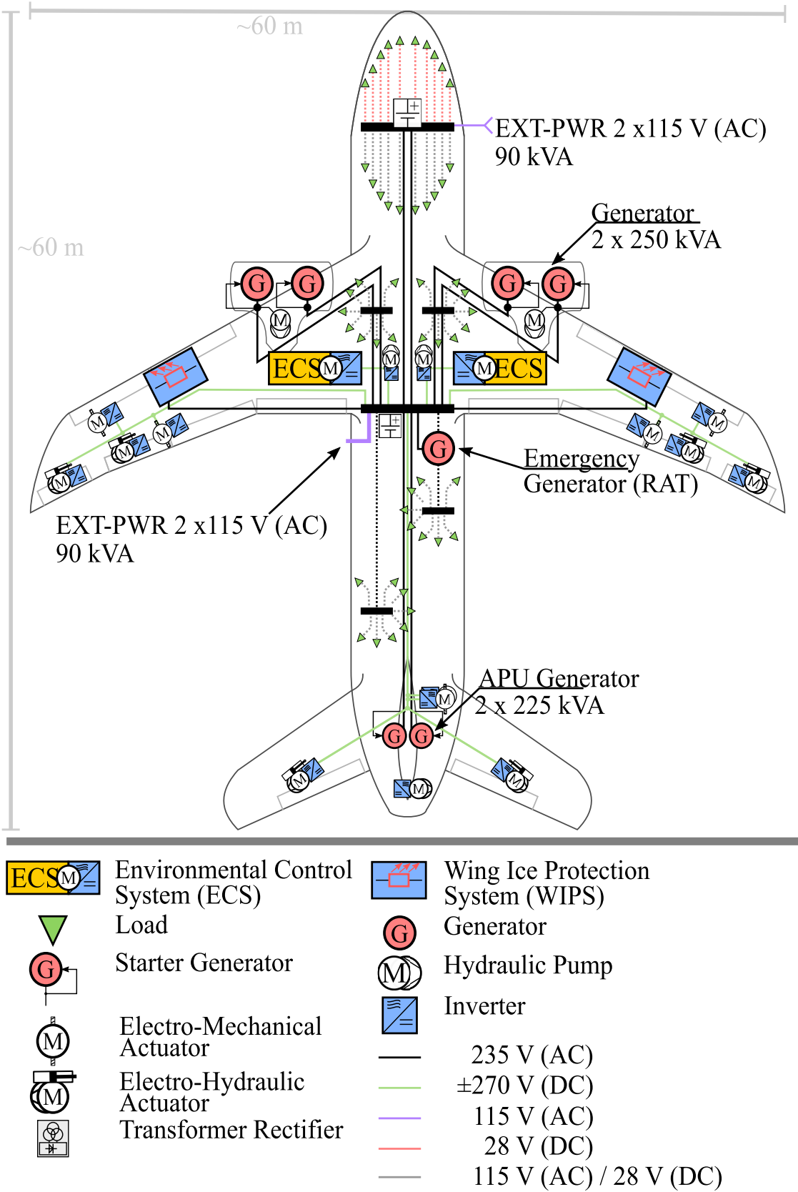
FIGURE 2. Electric schematic of MEA.
