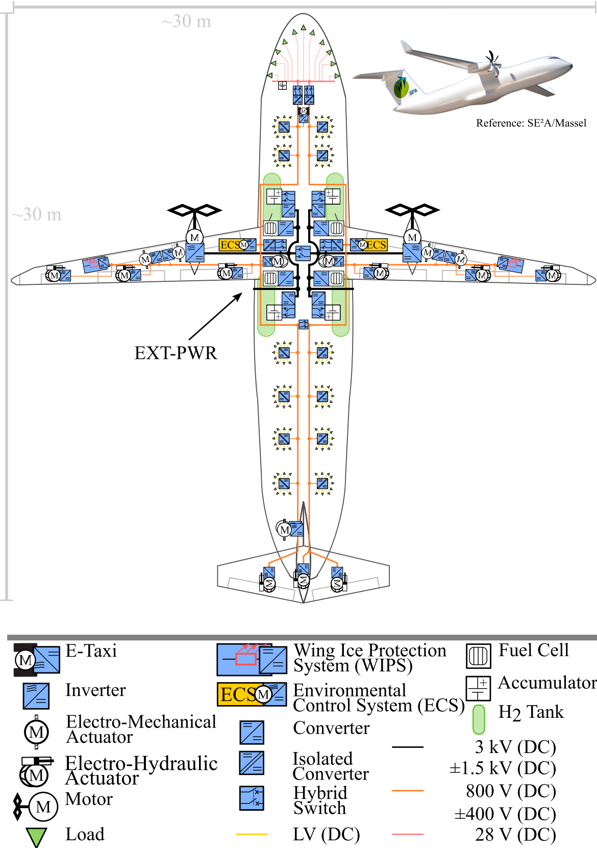
FIGURE 5. Electric schematic of AEA.
