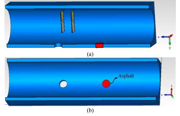
Fig. 9. Schematic of simulated structure. (a) Cross view. (b) Top view.
