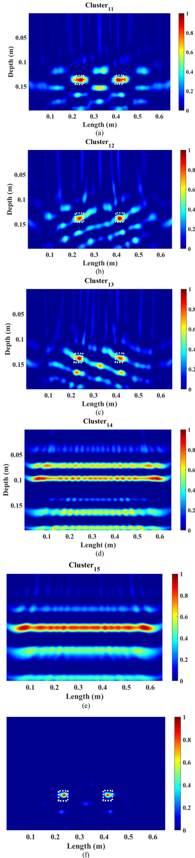
Fig. 7. Reconstructed image using 2-D SSA. (a) Cluster11. (b) Cluster12. (c) Cluster 13. (d) Cluster 14. (e) Cluster 15. (f) Modified 2-D SSA.
