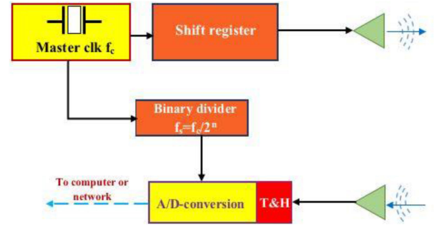
Fig. 12. Block diagram of M-sequence sensor.
