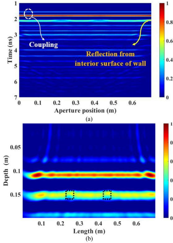
Fig. 5. (a) Raw data and (b) reconstructed image without any clutter removal.
