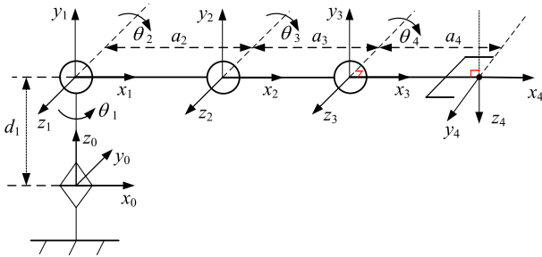
FIGURE 4. Link-pole coordinate system of the manipulator.
