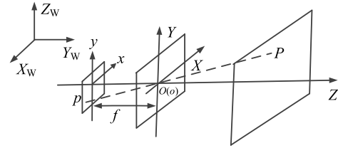
FIGURE 9. Schematic diagram of target positioning.
