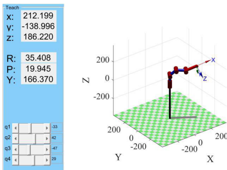
FIGURE 5. The orientation under random joint variables.
