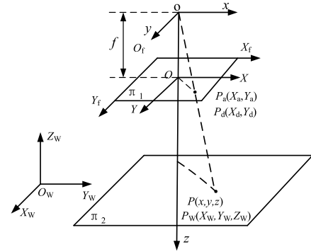
FIGURE 6. Relationship between the four coordinate systems.
