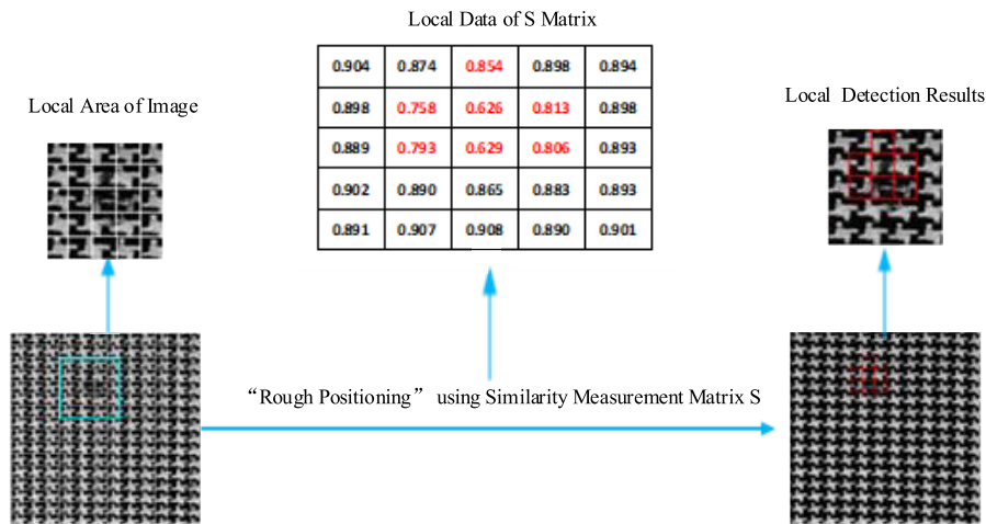
FIGURE 10. Schematic diagram of “rough-positioning.”
