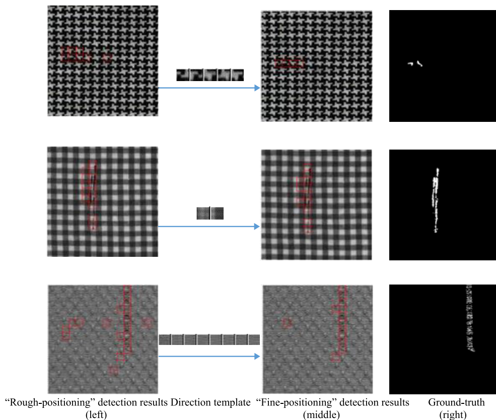
FIGURE 11. Results of “fine-positioning.”
