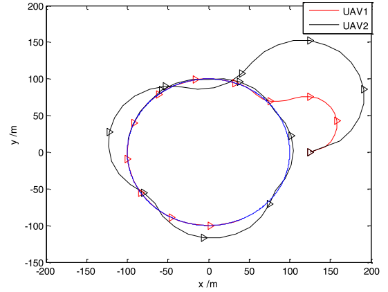
(a) The tracks of the traditional trajectory following algorithm
