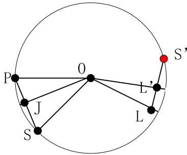
FIGURE 3. Schematic diagram of the CTAP algorithm.
