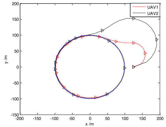
(b) The tracks of CTFAP algorithm
