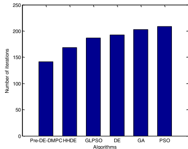
(b)Histogram of average iterations of all algorithms
