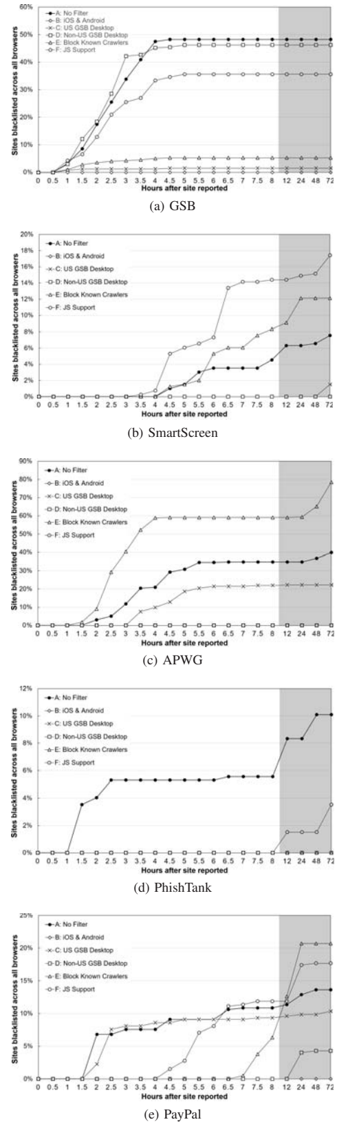
Fig. 4: Blacklisting over time by filter (full tests).
