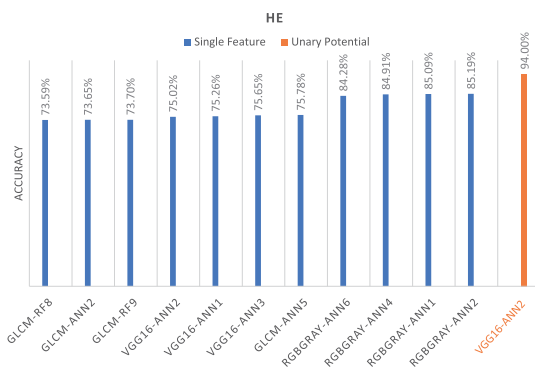
FIGURE 7. A comparison of image-level classification accuracies between selected feature-classifier combinations and the generated unary potential on the gastric HE validation set.
