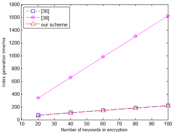
FIGURE 5. Encryption keyword time.
