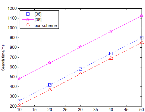
FIGURE 6. Search time.
