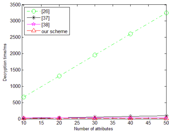
FIGURE 7. Decryption time.
