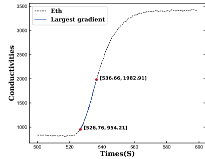
FIGURE 3. The reaction with Ethylene between 500s and 600s.
