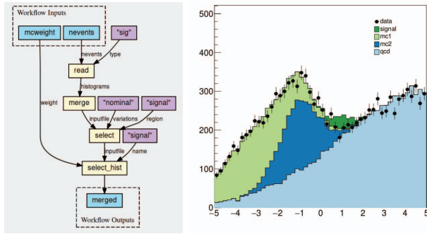
Fig. 2. A part of typical Beyond Standard Model particle physics search analysis expressed in the Common Workflow Language standard. An example plot simulating a hypothetical BSM signal ( signal ) over Standard Model background predictions ( mc1 , mc2 , qcd ) showing an excess of signal over data ( data ) at the pre-fit configuration of the model.
