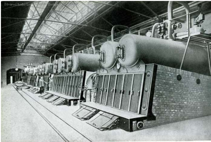
Fig. 20.: Boiler room of BVVV - Budapesti Villamos Városi Vasút Rt. (Budapest Electric Urban Train) in Kertész street, 1897 [15]
